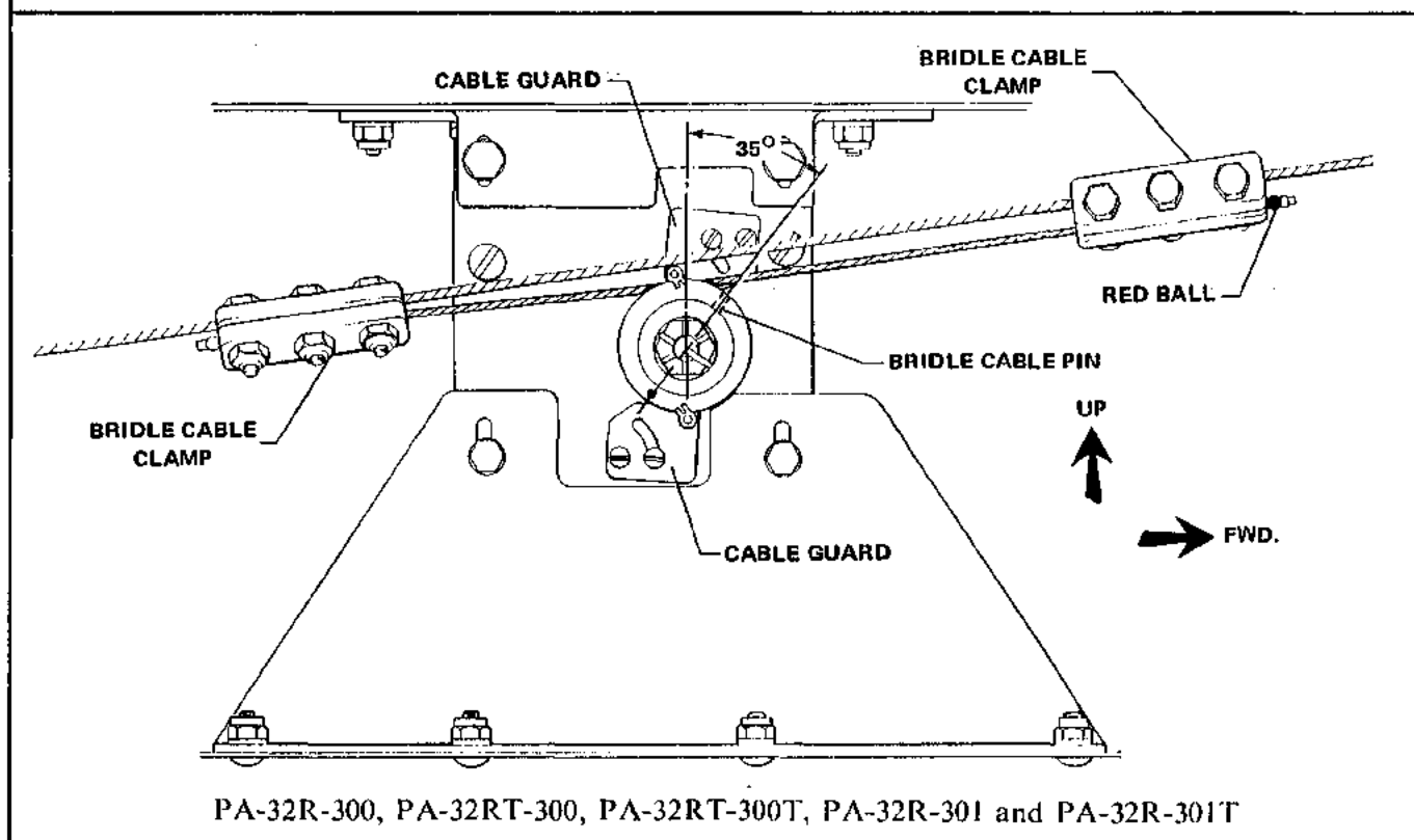
Figure 3-27. Roli Servo Installation
