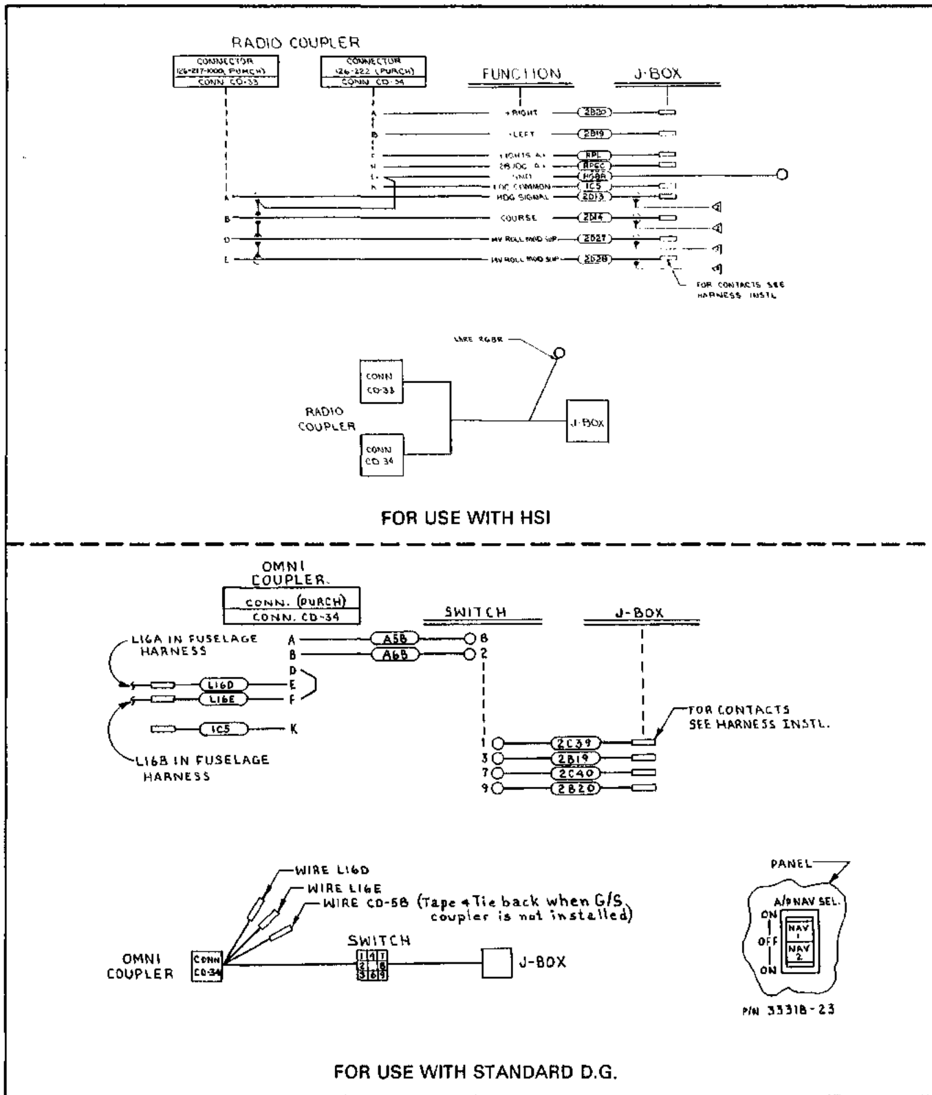
Figure 6-21. Radio Coupler Harness, PA-23-250 (Six Place)
