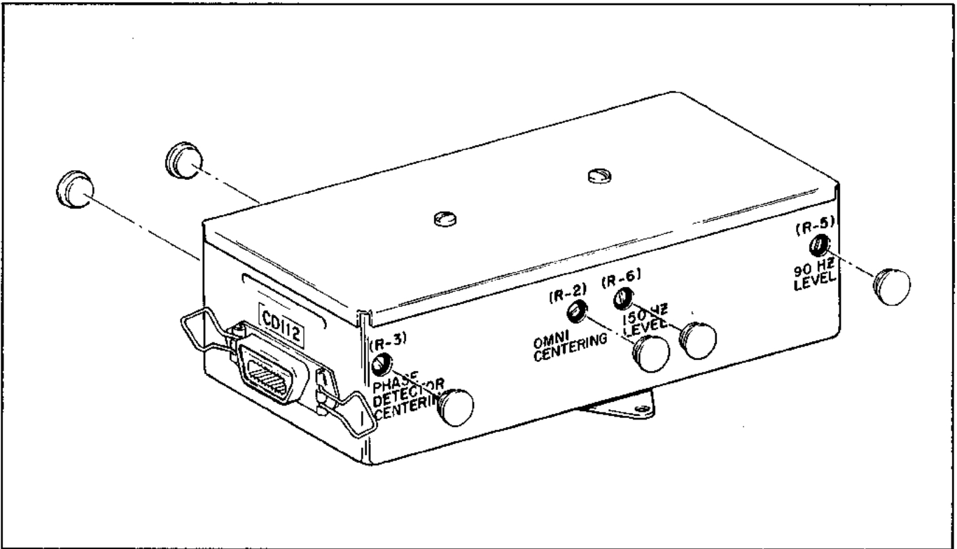
Figure 3-21. AltiMatic III C, NAV Converter (IC707)
