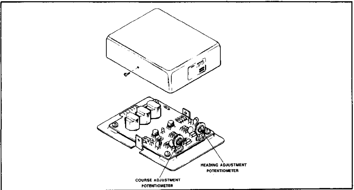
Figure 3-37. KA-52 Autopilot Adapter Installation
