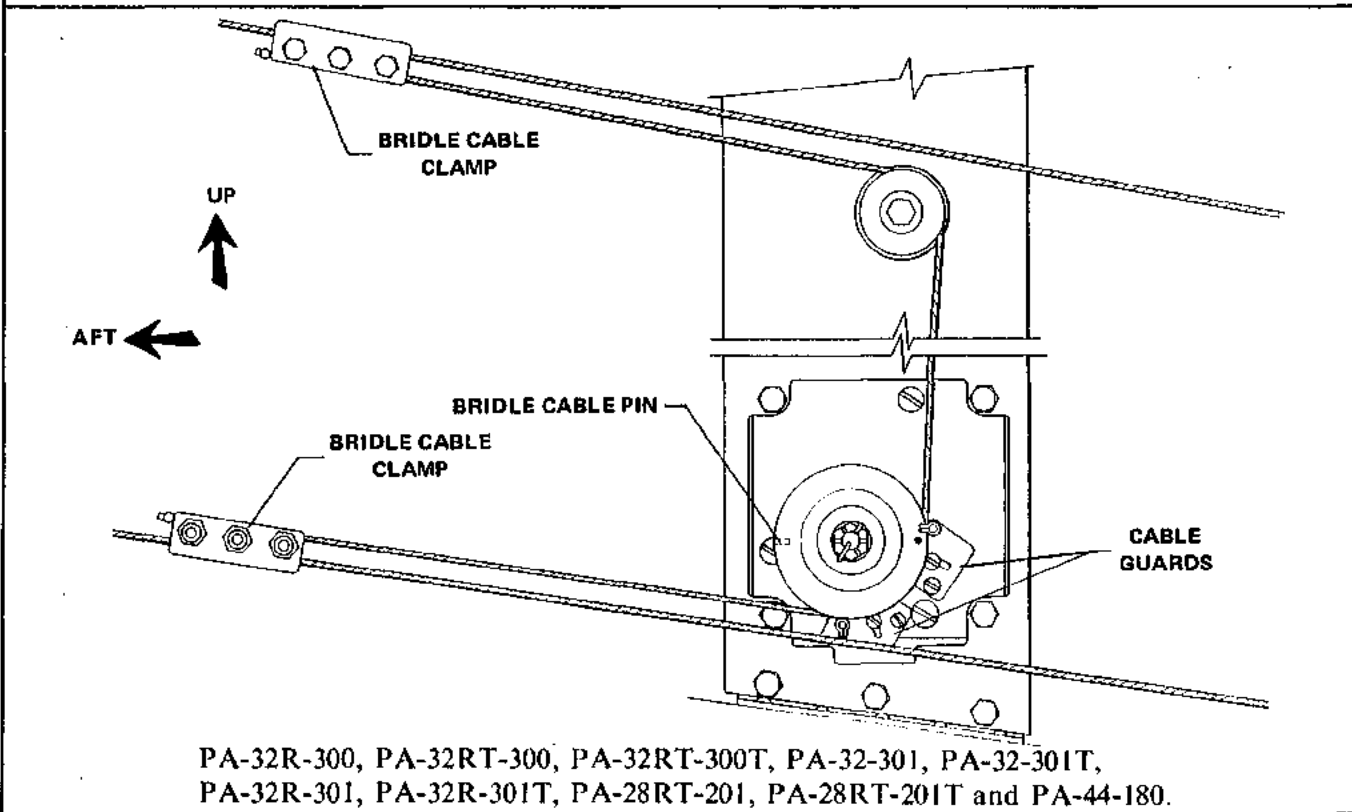
Figure 3-28. Pitch Servo Installation
